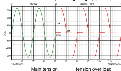
Phase attack (leading edge) principle
